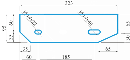
DRAWING DISTANCE BETWEEN HOLES
